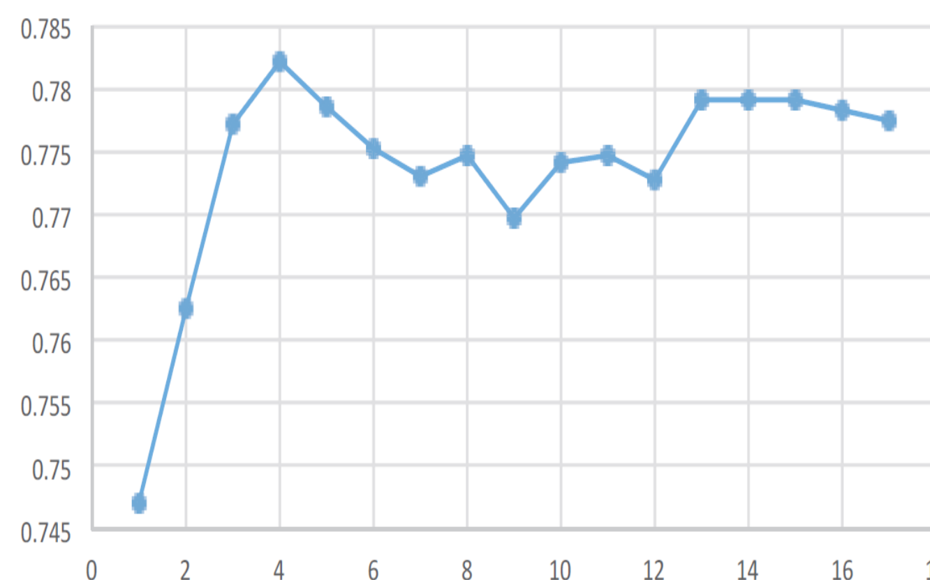
Figure 2. Effect of number of VOCs in algorithm (x-axis) on predictive accuracy (y-axis). It is apparent that the algorithm achieves its near maximal predictive accuracy (~78%) with only four VOCs (chromatogram segments) in the model, and then reaches a plateau. Addition of more VOCs to the predictive algorithm did not significantly improve its performance.
